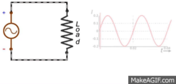
Alternating Voltage and Current
